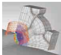
切屑模拟 Simulation of Chip Flow
