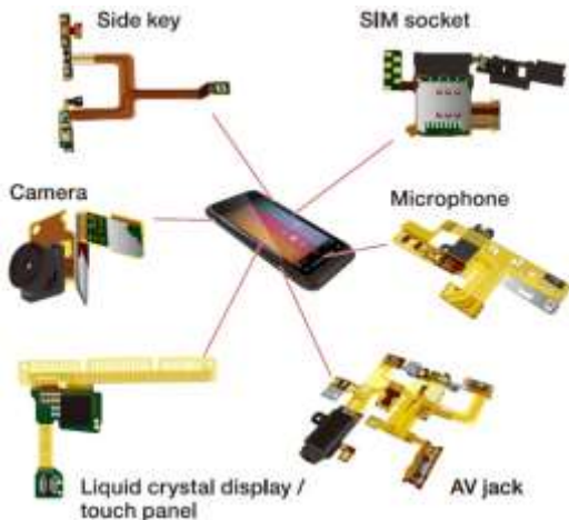
Flexible Printed Circuits (FPC)
